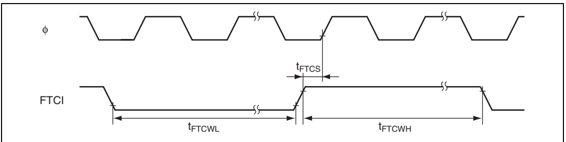
Figure 22.12 FRT Clock Input Timing
